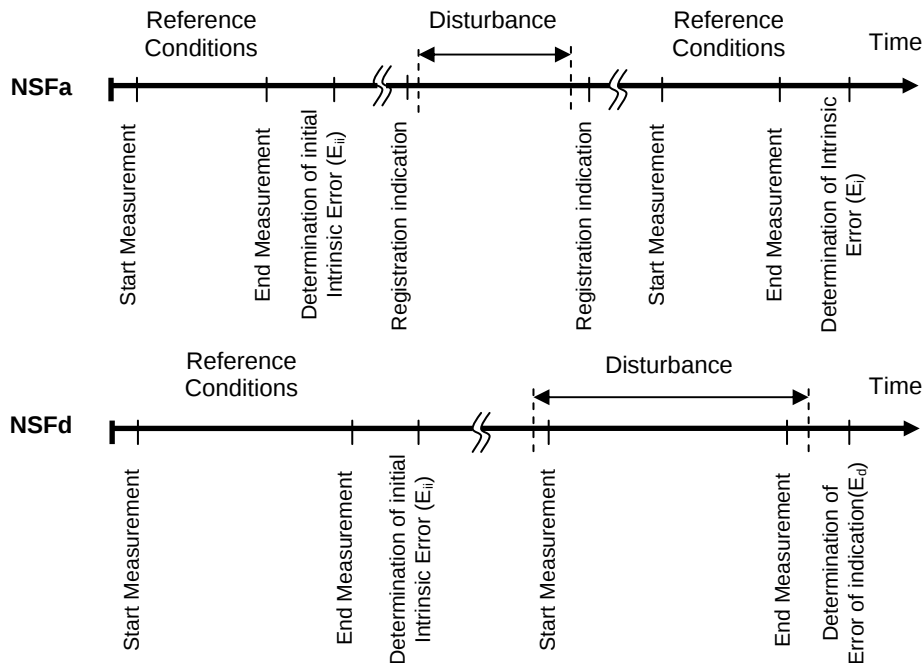
Figure 1 Time sequences for the two conditions: NSFa (No Significant Fault shall occur after the disturbance) and NSFd (No Significant Fault shall occur during the disturbance)
