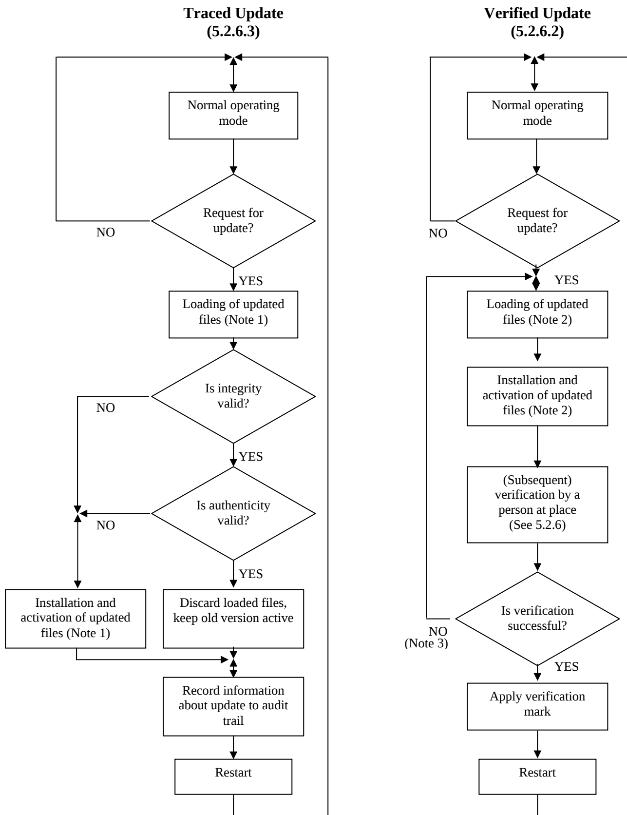
Figure 1: Software update procedure
